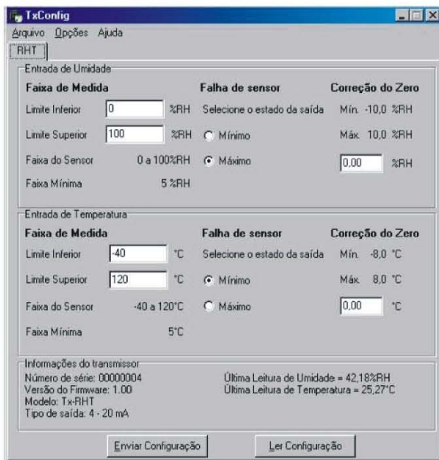
Tela principal do software TxConfig
